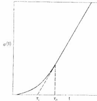
FIG. 4. The function \sigma(t) .
