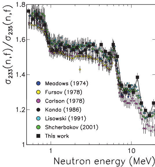
Fig. 2. Comparison of the present cross-section ratio ^{233}\text{U}/^{235}\text{U} (full squares and solid line, 20 bins per energy decade) with previous measurements [7–12]. For the data reported in ref. [9] information on the related uncertainties is not available.
