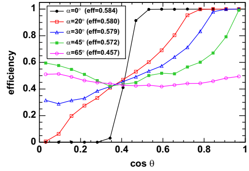
Fig. 4. Simulated detection efficiency for different values of the \alpha angle between the normal to the detectors and the neutron beam direction. The total detection efficiency for each case is indicated in the legend, with a statistical uncertainty of \pm 0.003 in all cases.
