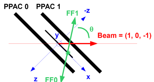
Fig. 2. Reference system used to calculate the emission angle \theta of the fission fragments.
