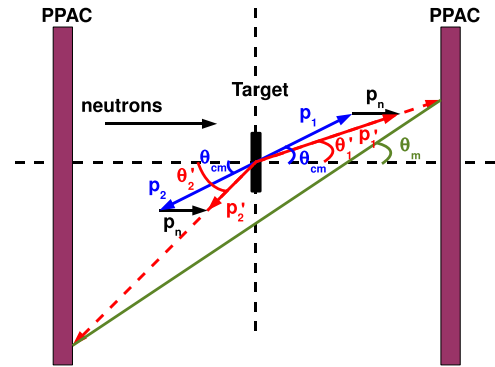
Fig. 5. Kinematics of a fission event detected by two PPACs.
