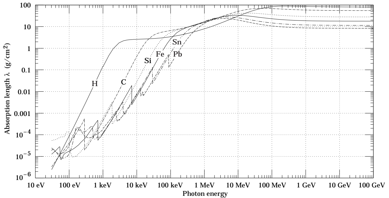
Figure 27.15: The photon mass attenuation length (or mean free path) \lambda = 1/(\mu/\rho) for various elemental absorbers as a function of photon energy. The mass attenuation coefficient is \mu/\rho , where \rho is the density. The intensity I remaining after traversal of thickness t (in mass/unit area) is given by I = I_0 \exp(-t/\lambda) . The accuracy is a few percent. For a chemical compound or mixture, 1/\lambda_{\text{eff}} \approx \sum_{\text{elements}} w_Z/\lambda_Z , where w_Z is the proportion by weight of the element with atomic number Z . The processes responsible for attenuation are given in not Fig. 27.9. Since coherent processes are included, not all these processes result in energy deposition. The data for 30 \text{ eV} < E < 1 \text{ keV} are obtained from http://www-cxro.lbl.gov/optical_constants (courtesy of Eric M. Gullikson, LBNL). The data for 1 \text{ keV} < E < 100 \text{ GeV} are from http://physics.nist.gov/PhysRefData , through the courtesy of John H. Hubbell (NIST).
