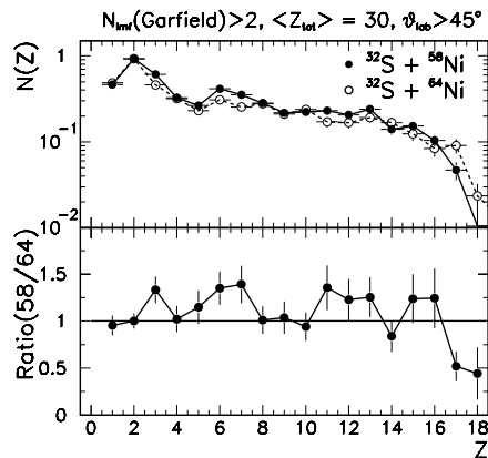
Fig. 11. Charge distribution (upper panel) in the reactions ^{32}\text{S}+^{58}\text{Ni} and ^{32}\text{S}+^{64}\text{Ni} , for events with at least three IMFs detected in GARFIELD. In the lower panel, the ratio of the two charge distributions is shown. Both charge distributions are normalized to the total number of events.
