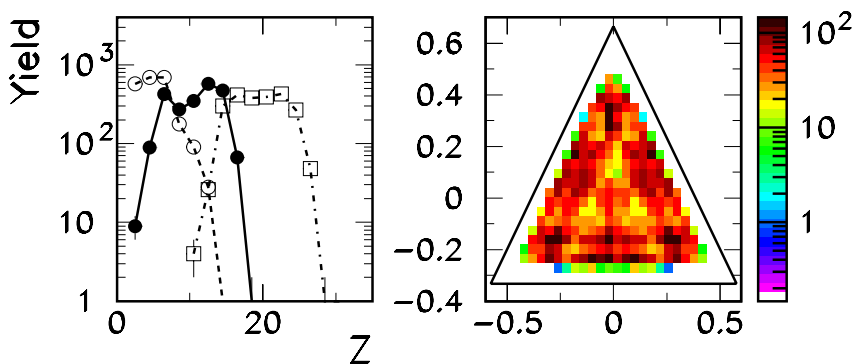
Fig. 10. Same as Fig. 7, but simulated by SMM statistical multi-fragmentation model. Both charge distributions are normalized to the total number of events.
