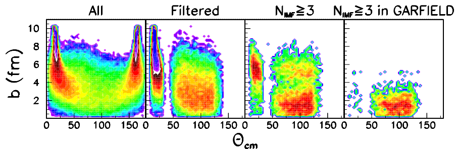
Fig. 4. CMD model predictions for the reaction ^{32}\text{S} + ^{58}\text{Ni} at 11 A MeV. Upper panels: the total event distribution as a function of the impact parameter b and of the \theta angle in the centre-of-mass system is shown without any experimental constraint (first panel), after the application of the experimental acceptance filter (second panel), when the additional condition of at least three detected IMFs is required in the whole apparatus (third panel) or in GARFIELD only (forth panel). Bottom panel: a scatter plot of the correlation between charge of emitted IMFs and impact parameter is shown for the (experimental) events corresponding to the forth-upper panel.
