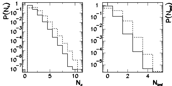
Fig. 2. ^{32}\text{S} + ^{58}\text{Ni} reaction at 11 A MeV. Experimental charged-particle (left) and IMF (right) multiplicity distributions. The yields are normalized to their sum. The dashed lines represent the distributions of products detected by the whole apparatus, the solid lines the distributions of those detected by GARFIELD only.
