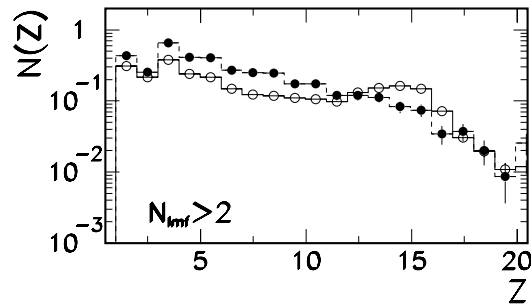
Fig. 6. ^{32}\text{S} + ^{58}\text{Ni} reaction at 11 A MeV. Filtered CMD charge distribution for events with at least three IMFs: open symbols refer to events detected in the whole apparatus, full symbols to events detected in GARFIELD. As shown in Fig. 4, this results in \langle b \rangle \approx 2 fm. Both charge distributions are normalized to the total number of events.
