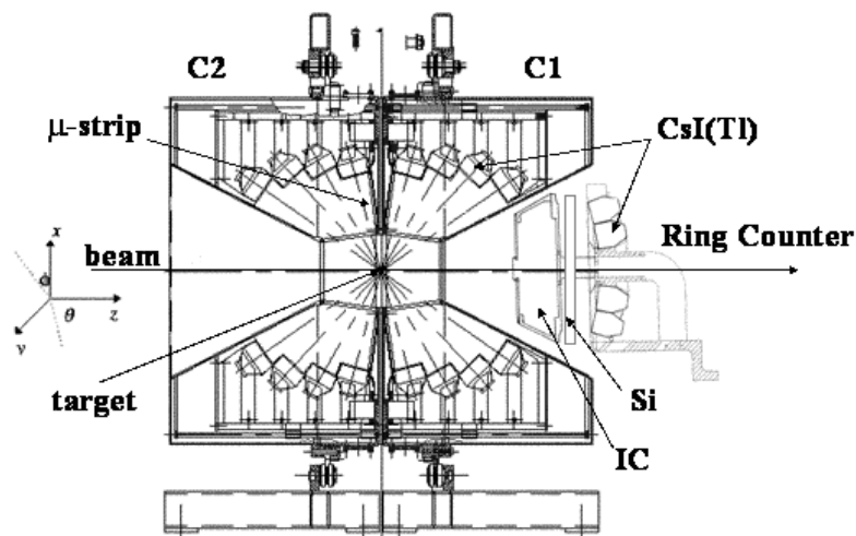
Fig. 1. Schematic drawing of the experimental apparatus: the two drift chambers (C1 and C2) are located back to back, with the target in between, while the annular detector is positioned in the forward direction with respect to the beam.
