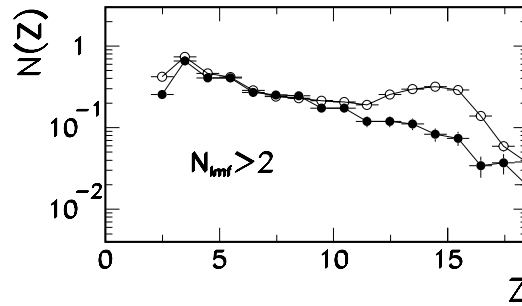
Fig. 5. ^{32}\text{S} + ^{58}\text{Ni} reaction at 11 A MeV. Charge distribution of IMFs detected in the whole apparatus (open symbols) and in GARFIELD (full symbols) for events with at least three IMFs. Both charge distributions are normalized to the total number of events.
