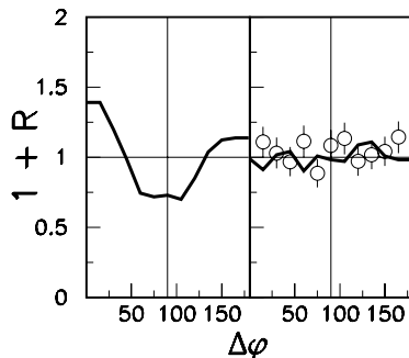
Fig. 3. ^{32}\text{S} + ^{58}\text{Ni} reaction at 11 A MeV. Azimuthal correlation function for \alpha -particles detected in GARFIELD, gated by three IMFs detected at large angles in the GARFIELD drift chamber. Left panel: correlation function calculated with the sequential statistical model code GEMINI for \langle L \rangle = 48 \hbar . Right panel: experimental data and GEMINI calculation for \langle L \rangle = 10 \hbar .
