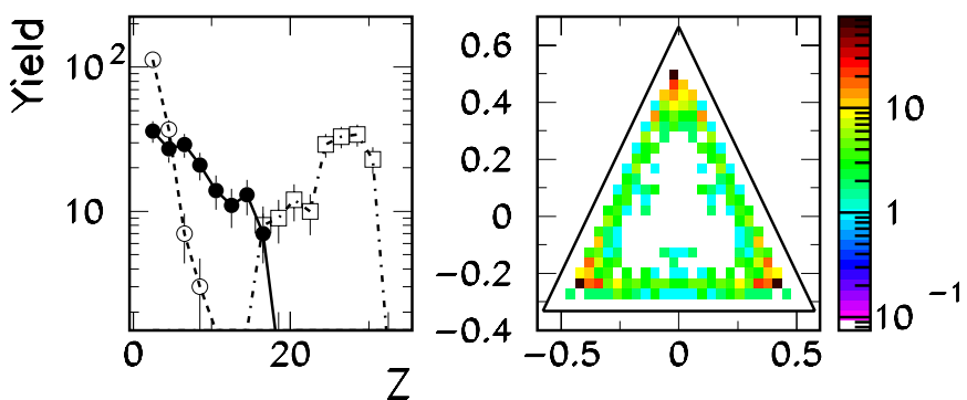
Fig. 9. Same as Fig. 7, but simulated by GEMINI statistical model with \langle L \rangle = 48 \hbar . Both charge distributions are normalized to the total number of events.
