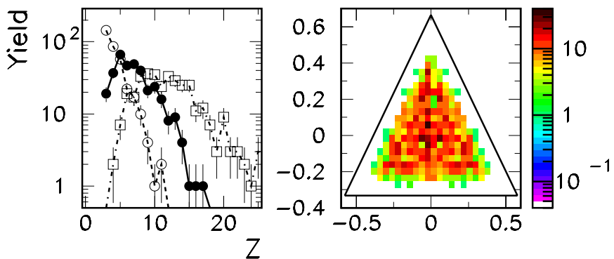
Fig. 8. Same as Fig. 7, but simulated by CMD dynamical model. Both charge distributions are normalized to the total number of events.
