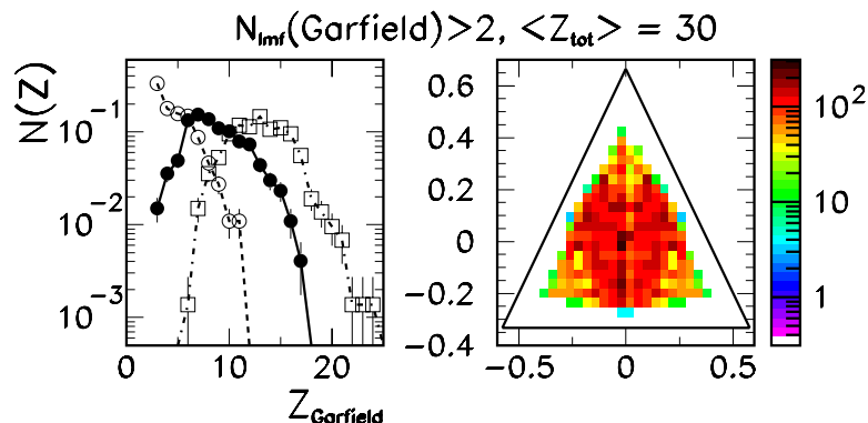
Fig. 7. ^{32}\text{S} + ^{58}\text{Ni} reaction at 11 A MeV. Charge distribution of the three largest IMFs detected in each event (left panel) and relative Dalitz plot for the experimental data. Both charge distributions are normalized to the total number of events.
