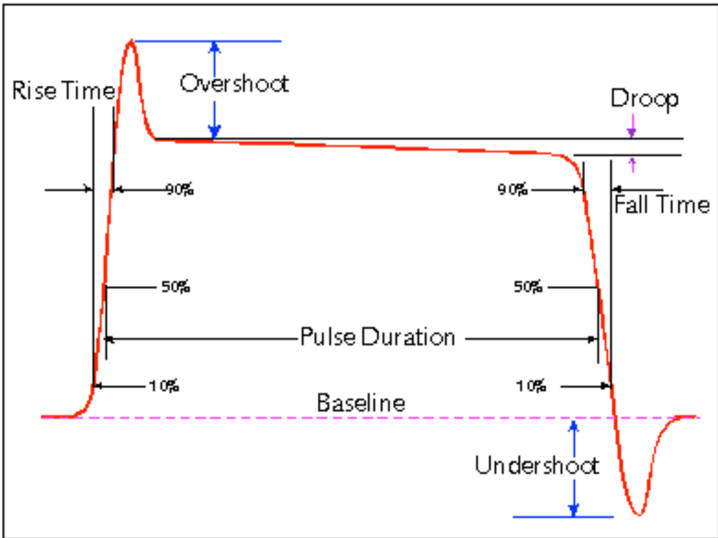
representative pulse waveform
