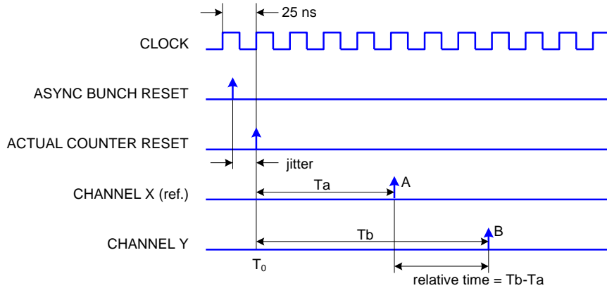
Fig. 2.9: Relative Time measurement
