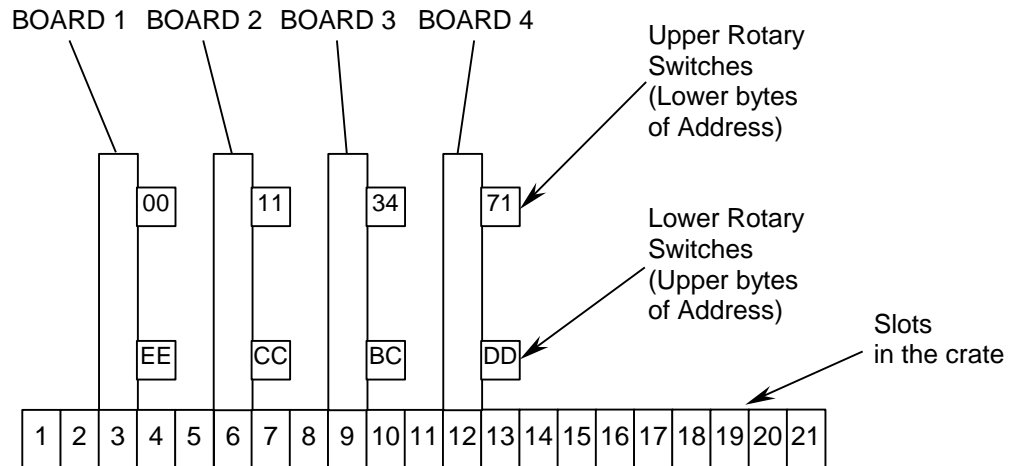
Fig. 4.2: MCST/CBLT Addressing Example
