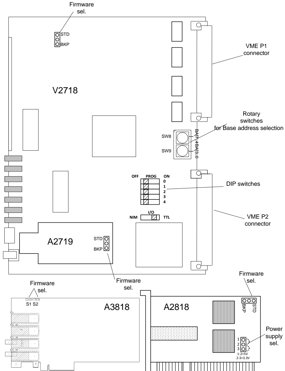
Fig. 38: Component Location
