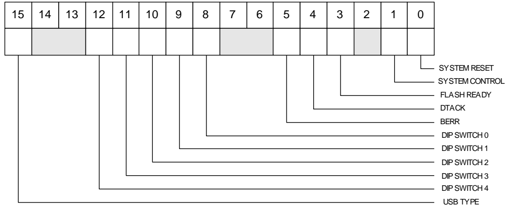
Fig. 6: Status Register
