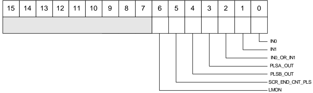
Fig. 11: Input register
