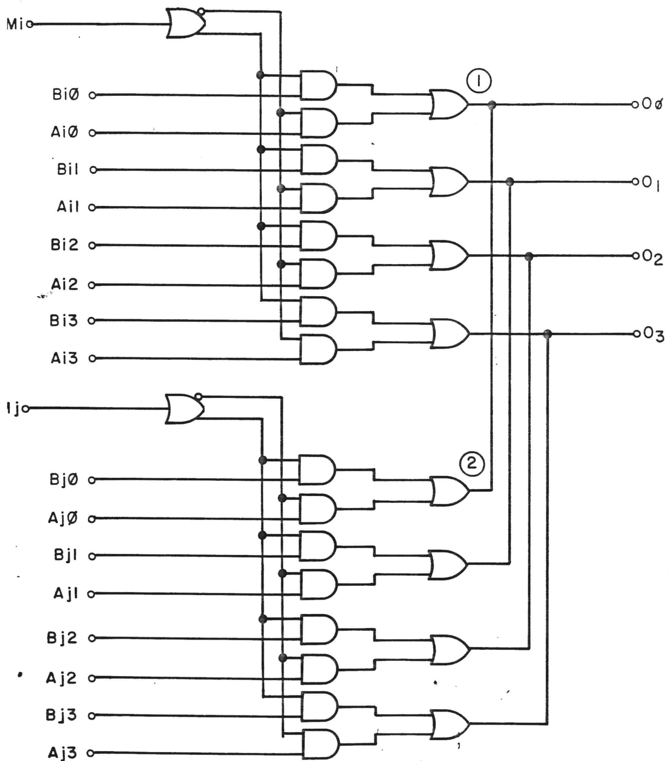
HLM 440 SIMPLIFIED SCHEMATIC
