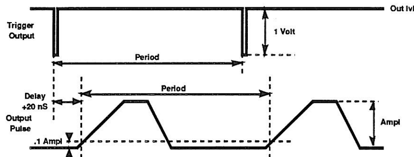
Nominal Trigger Output Widths in Normal Trigger Mode
